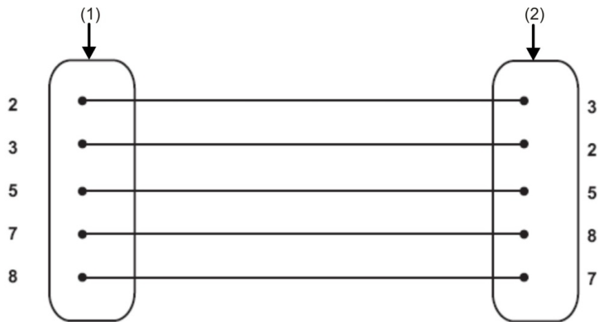
Figure 17: RS-232 cable connections
