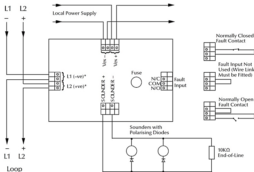
Figure 1 Sounder Control Unit with Isolator Wiring Diagram
